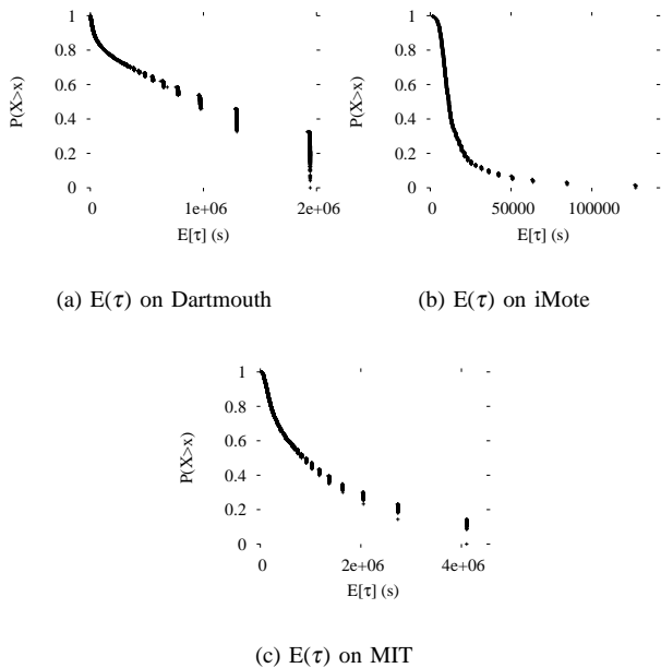
Fig. 1. CDF of mean inter-contact times E(\tau) .
