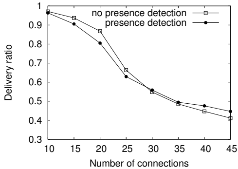
Figure 4: Worst case network performance.
